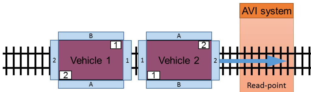
Figure 6-1 AVI system monitoring single tracks
