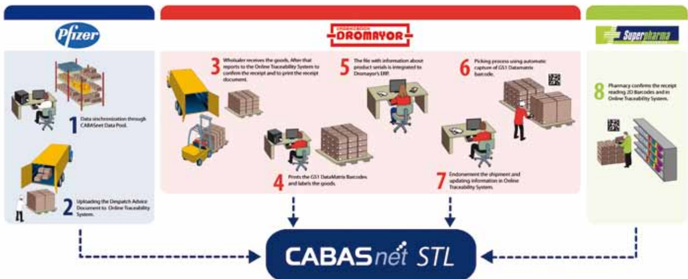
Figure 1: Pilot process
