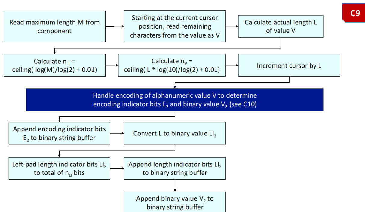
Figure 8-9 C9: Encode a variable-length alphanumeric value, referring to flowchart C10 for additional details
