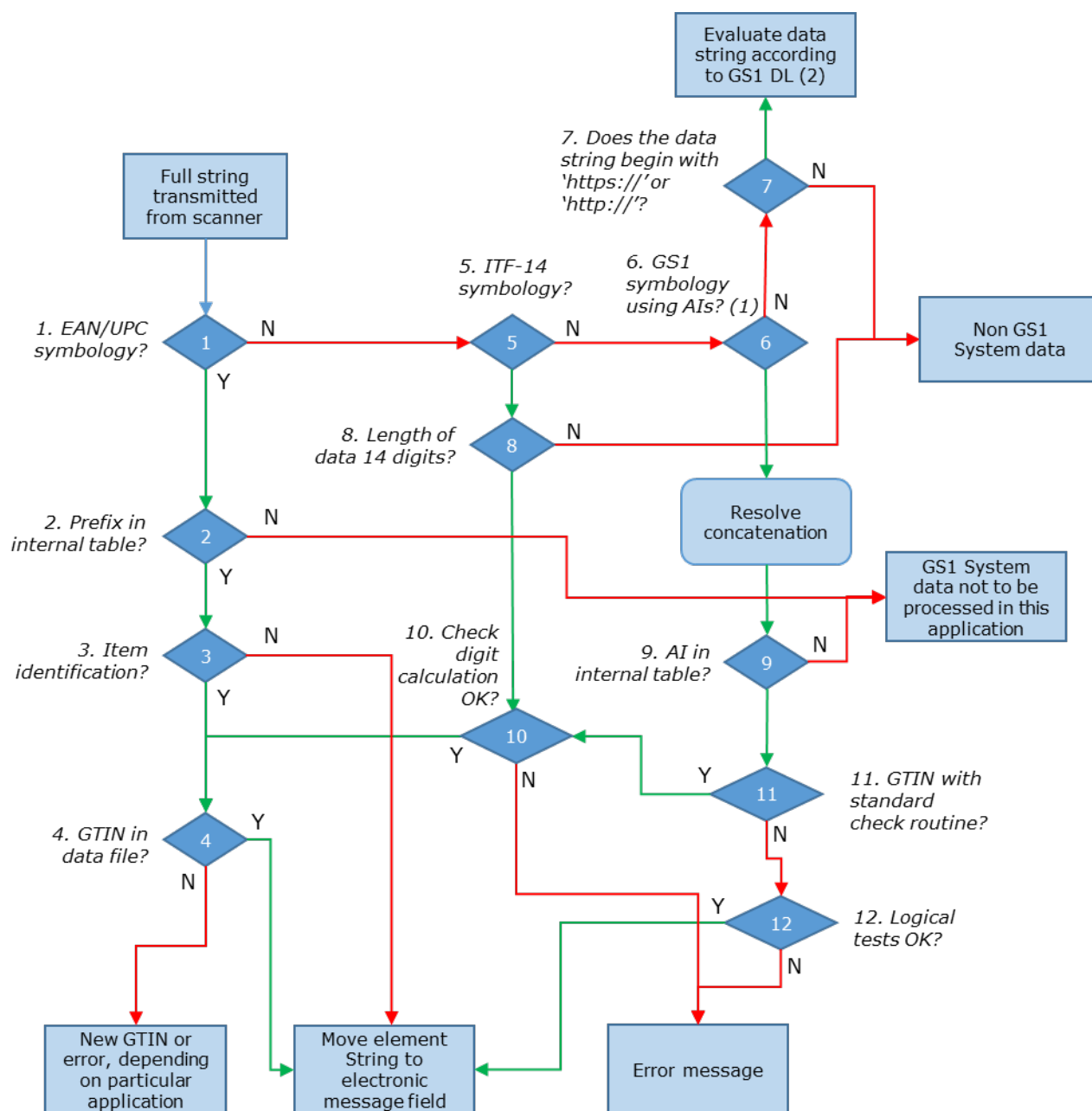
Figure 7-2 Test procedure
